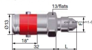
Socket, UNF male thread
