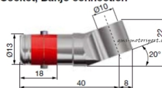
Socket, Banjo connection
